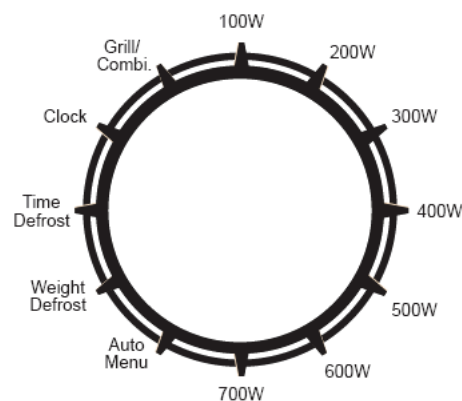
MULTI-FUNCTION SWITCH
